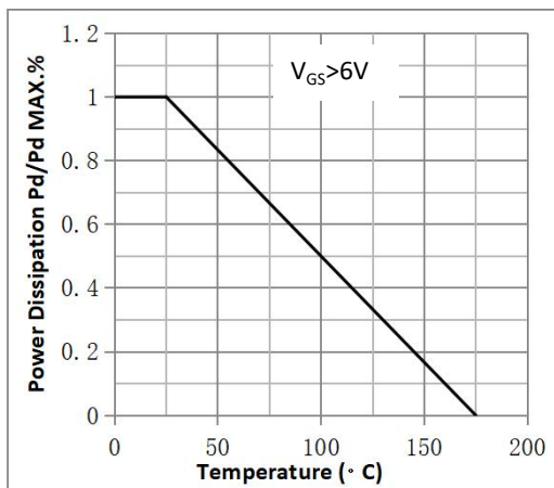
Fig.3 Power Dissipation
