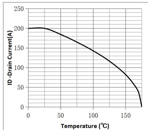
Fig.12 ID vs. Junction Temperature ③
